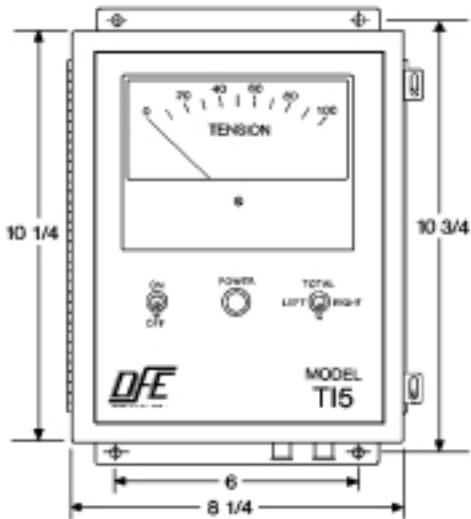
ENCLOSURE
