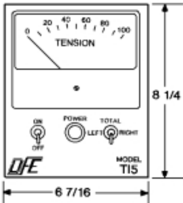
REMOTE PANEL
